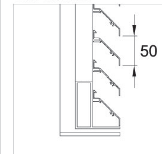
Cill detail
