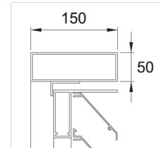
Head detail
