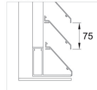
Cill detail
