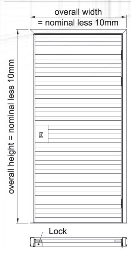
Single door
